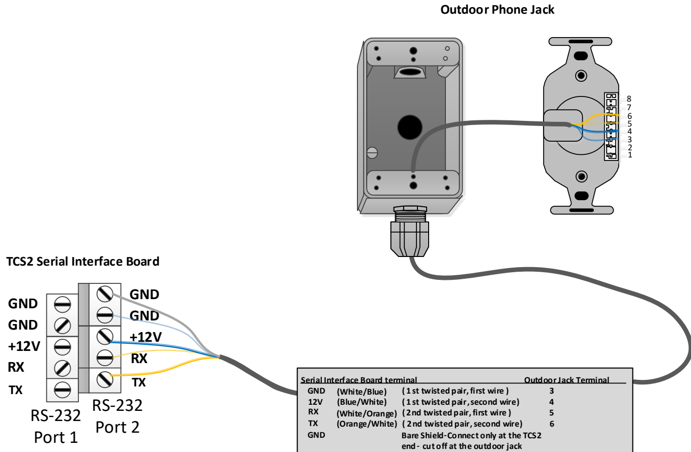
Figure 11: TCS2 Jack Wiring
