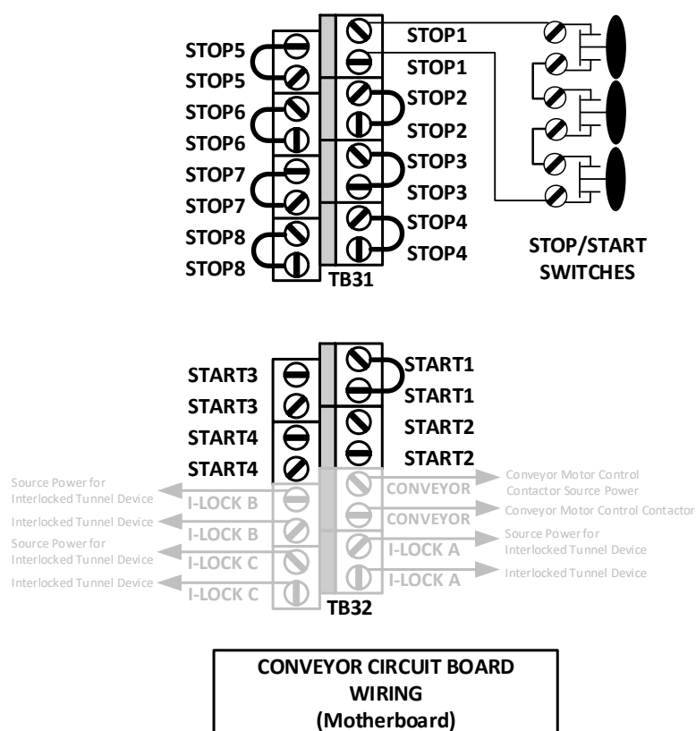
Figure 15: Single Stop Button 2-Wire "Daisy Chain" Wiring Method
