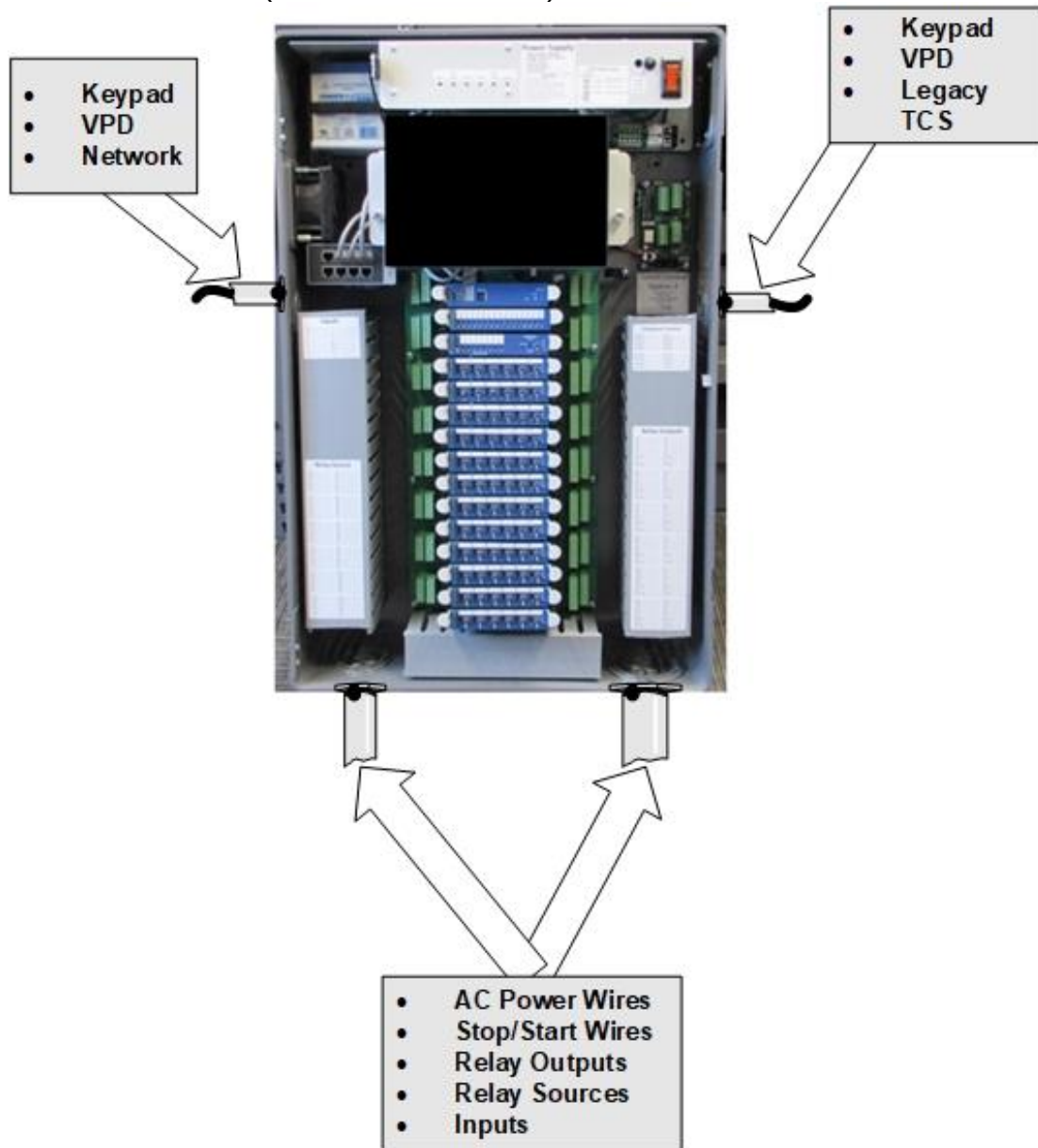
Figure 1: TCS2 Box with Conduits
