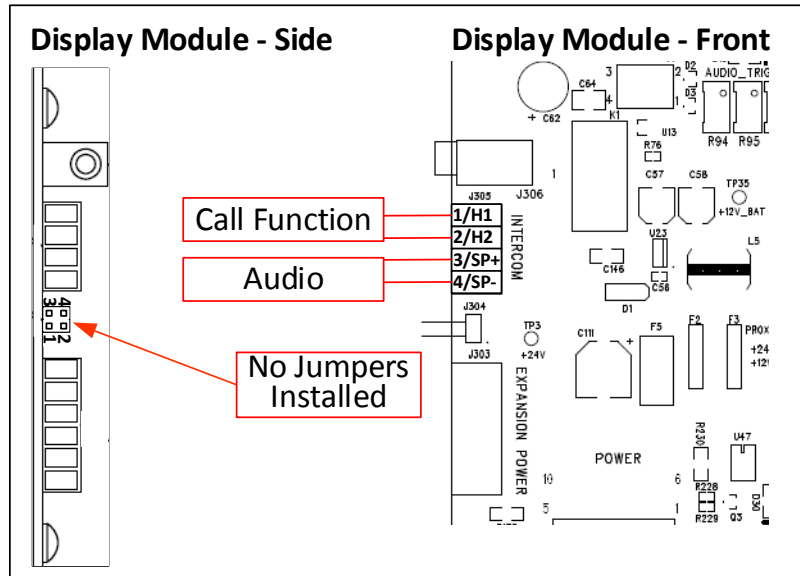
Figure 32. Four-Wire Intercom Configuration
