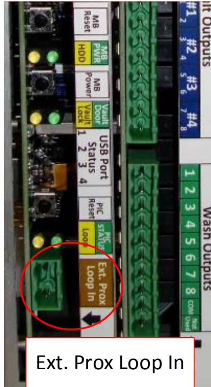
Figure 29. External Prox Loop Lead-In Connections
