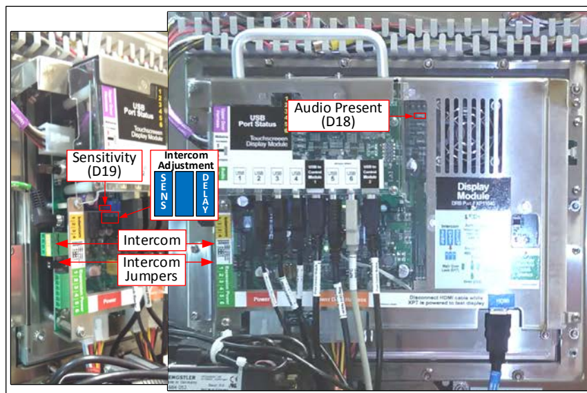
Figure 31. Intercom Component Locations on the Display Module
