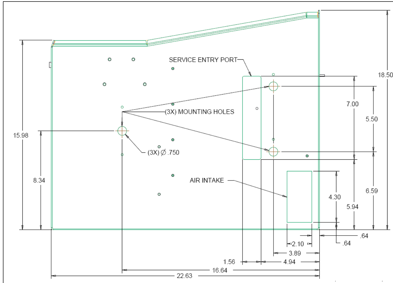
Figure 38. Bottom View of the XPT (case only)
