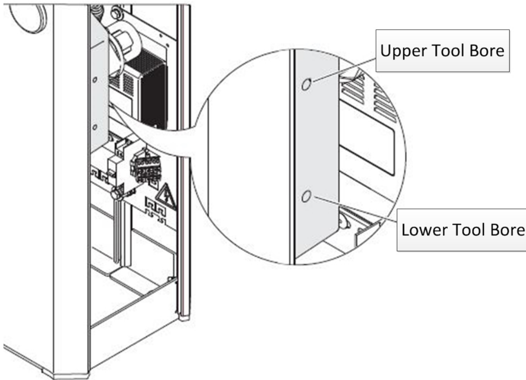
Figure 57. Open Gate Using Upper Tool Bore
