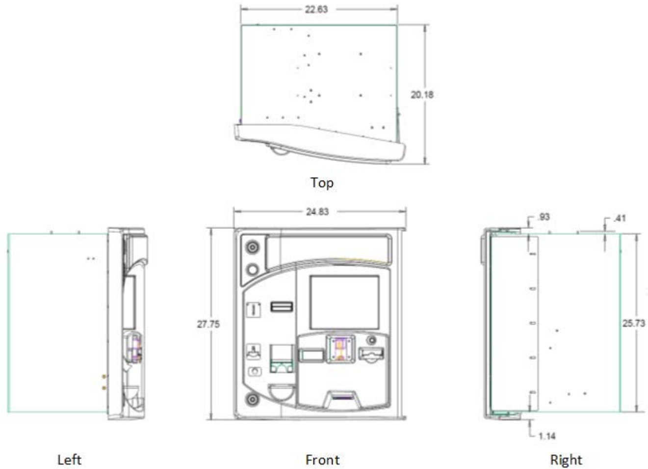
Figure 40. Brick-In XPT (No Plastic Shroud)
