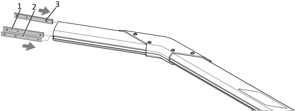
Figure 59. Install Slot Nuts
