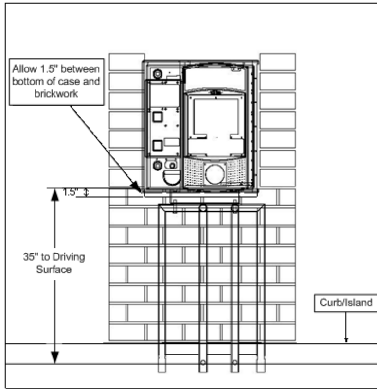
Figure 21. Bricked-In XPT with Adaptor Plate and Standard Base Frame
