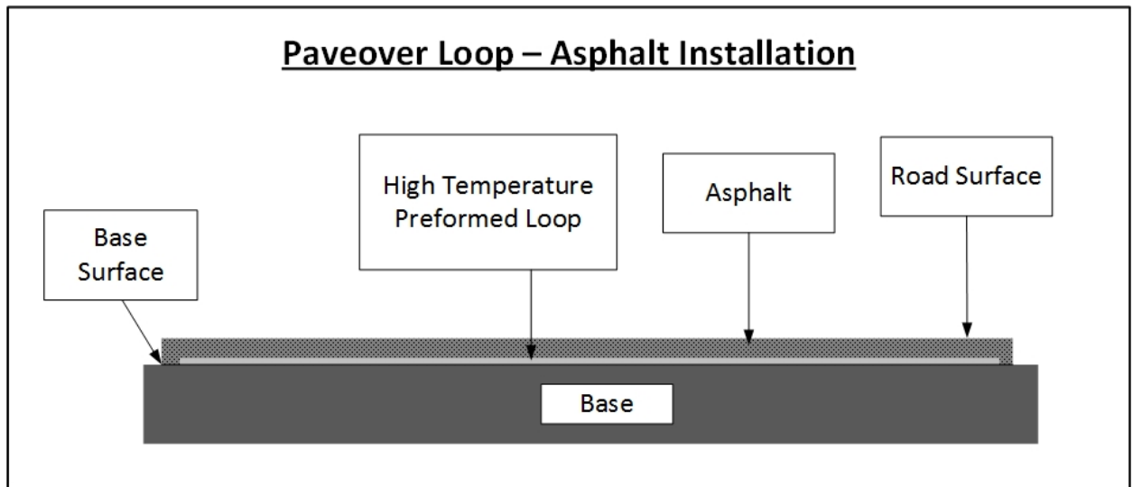
Figure 55. Pave-over Loop - Asphalt Installation
