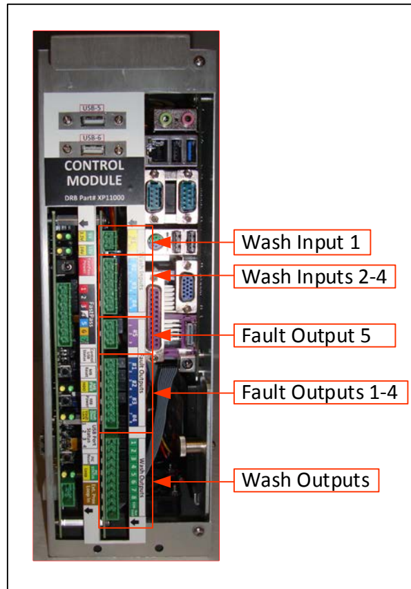
Figure 25. Control Module Input/Output Connectors
