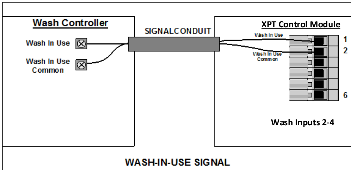
Figure 67. Wash in Use Circuit
