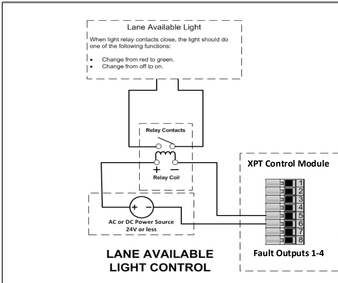
Figure 65. Lane Available Light Output Circuit
