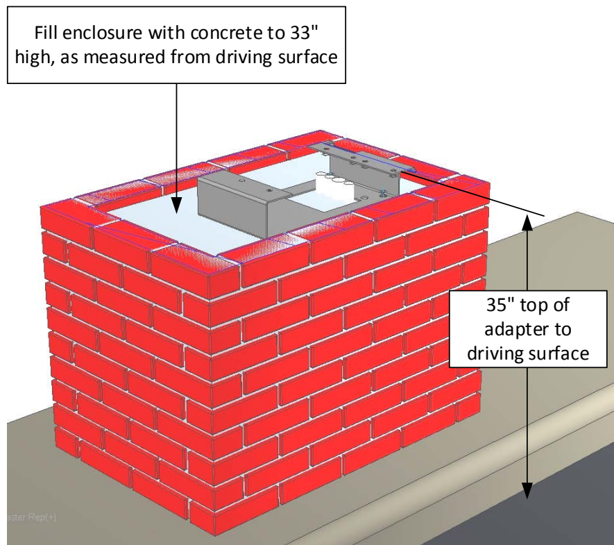
Figure 18. Fill Brick Enclosure with Concrete
