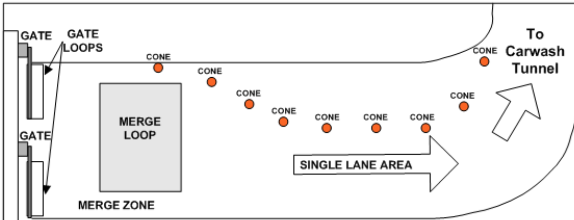
Figure 5. Merge Loop Location for Site with Two Gates
