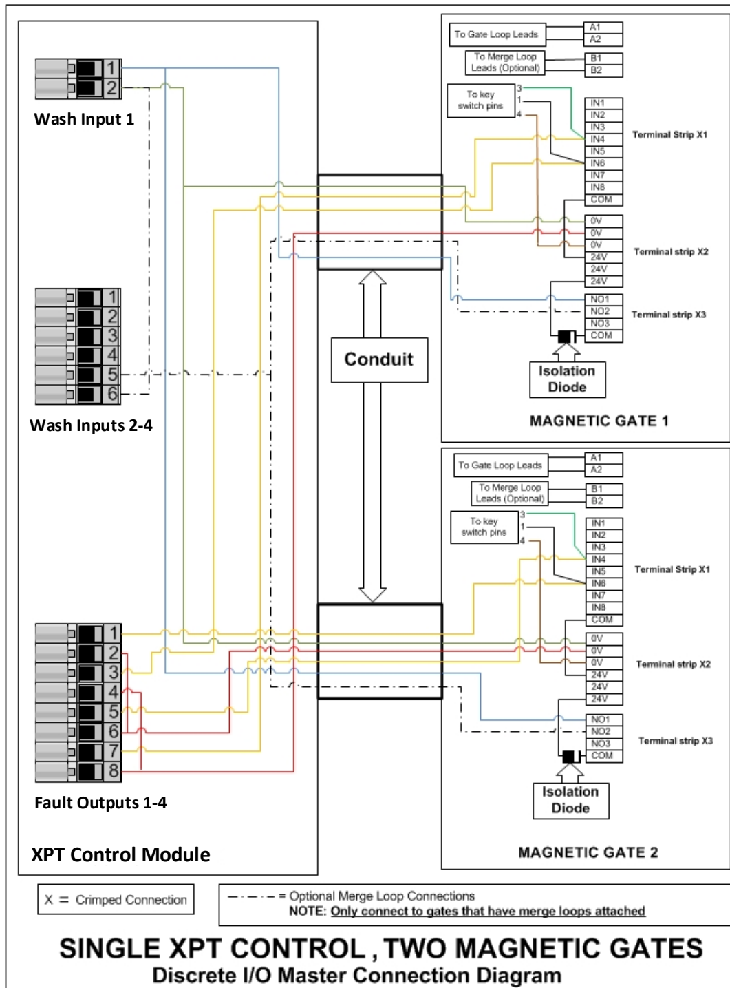
Figure 64. Two Magnetic Gates Controlled by a Single XPT - Master Connection Diagram
