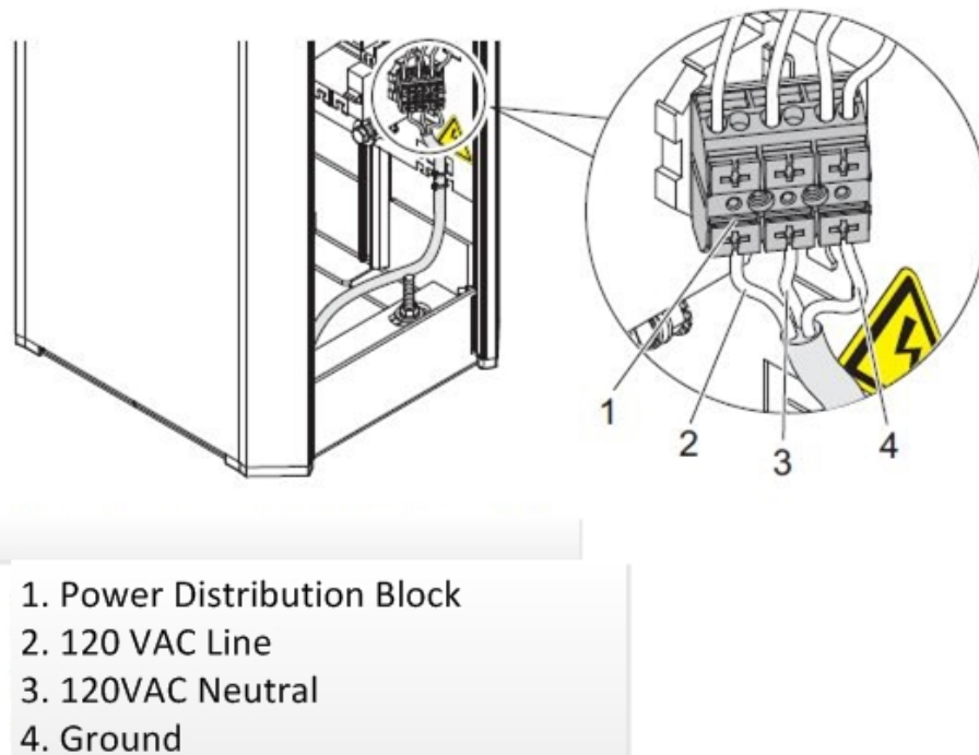
Figure 45. Gate Power Wiring
