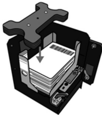
Figure 37. Card Dispenser Loading
