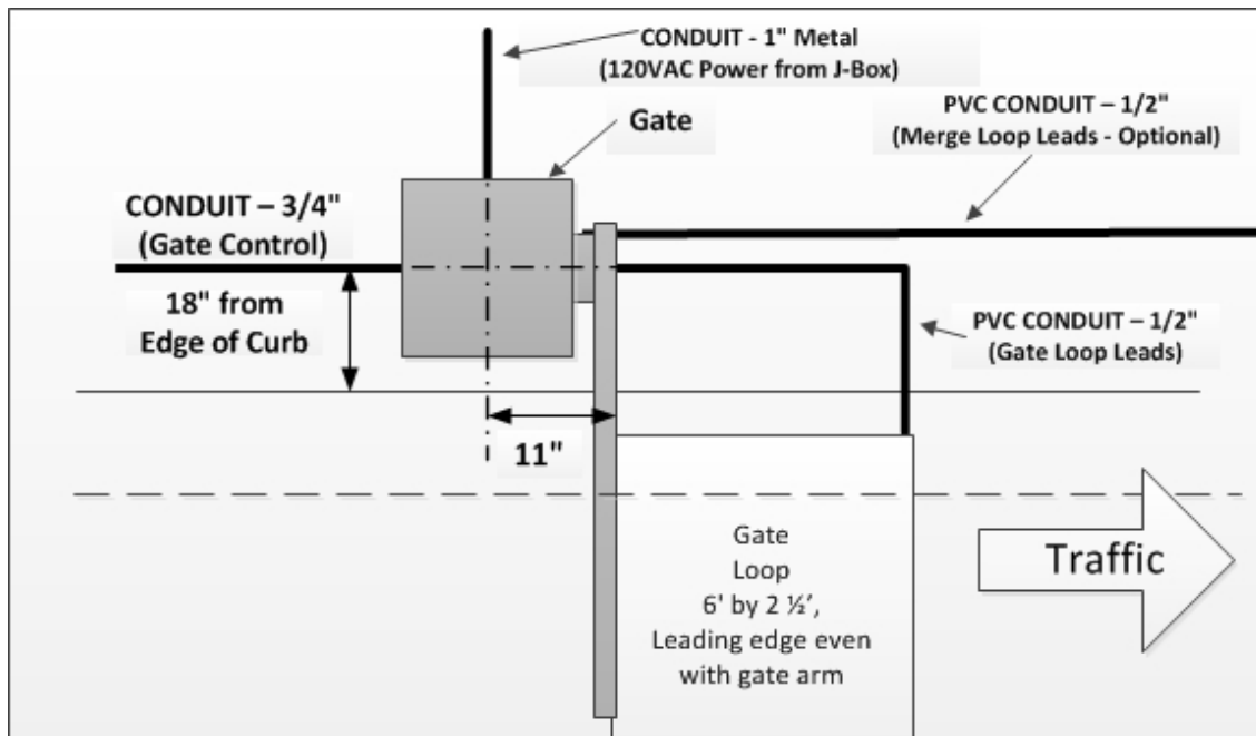
Figure 4. Gate Installation
