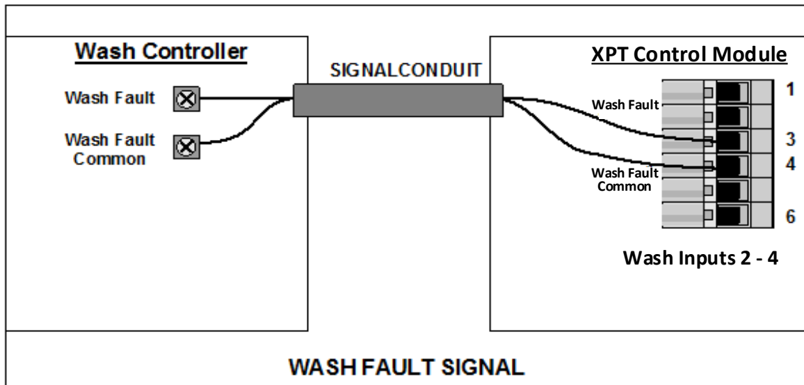
Figure 68. Wash Fault Circuit
