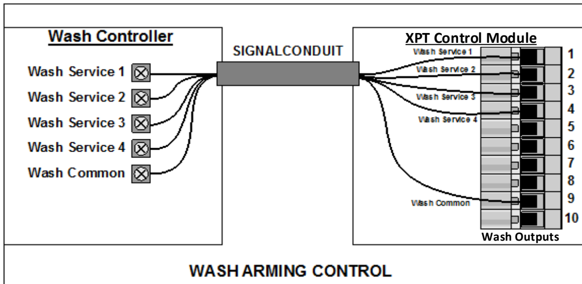
Figure 66. Wash Service Output Circuits
