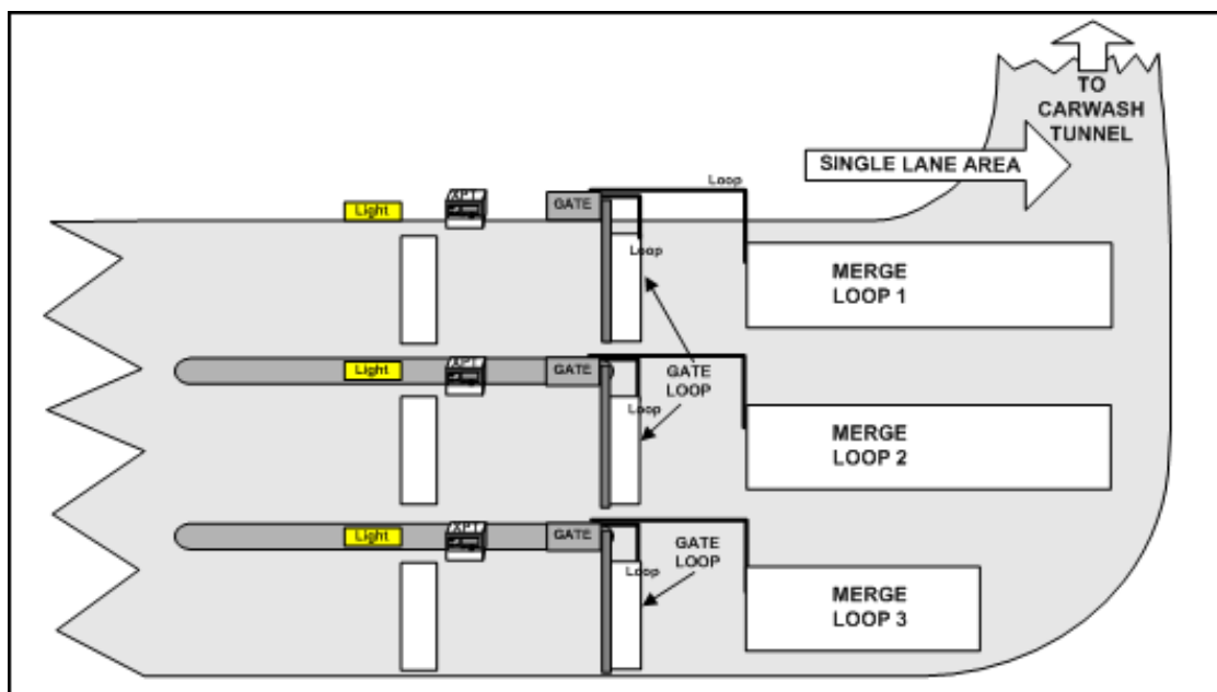
Figure 6. Merge Loop Locations for Sites with More than Two Gates
