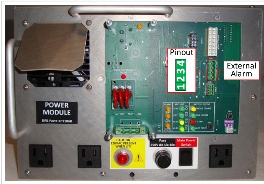
Figure 36. Power Module External Alarm Connection
