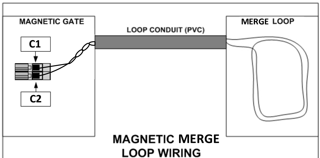
Figure 49. Magnetic Merge Loop Wiring
