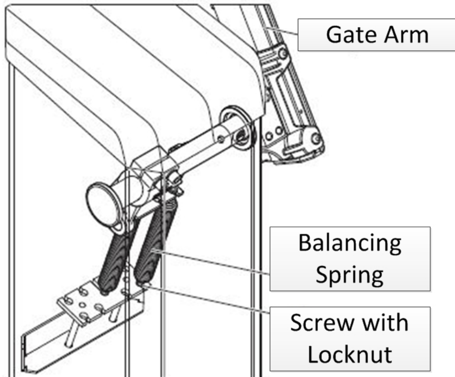
Figure 63. Balancing Springs
