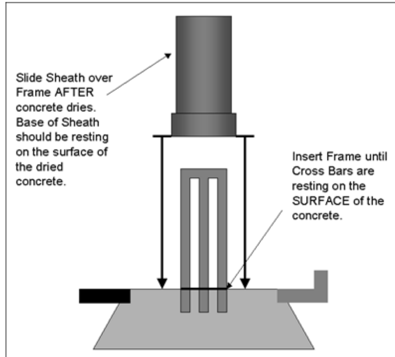
Figure 9. Frame and Sheath Installation
