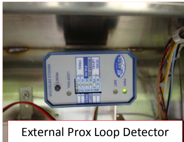
Figure 28. Optional External Prox Loop Detector
