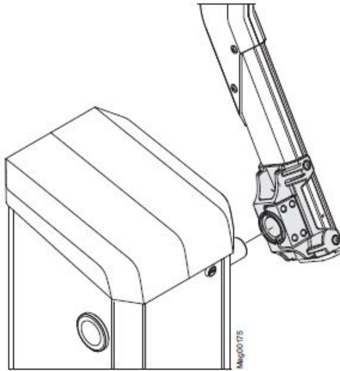
Figure 62. Install Flange onto the Flange Shaft
