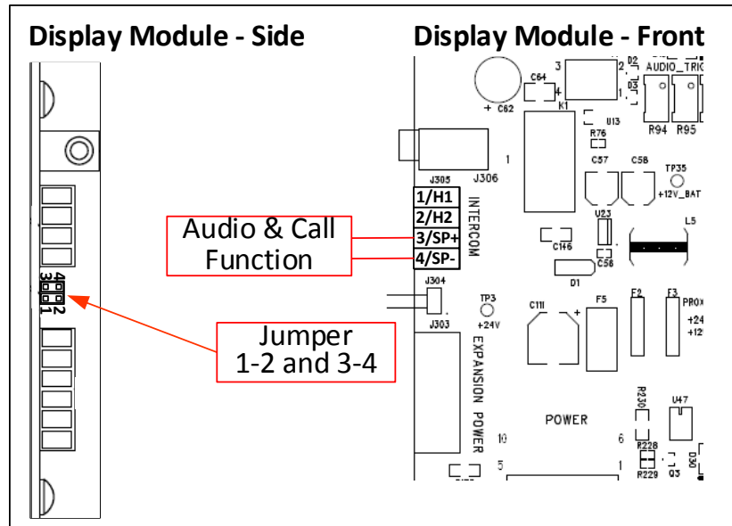
Figure 34. Two-Wire Intercom Configuration
