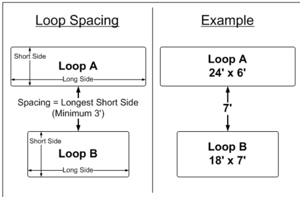
Figure 51. Merge Loop Separation
