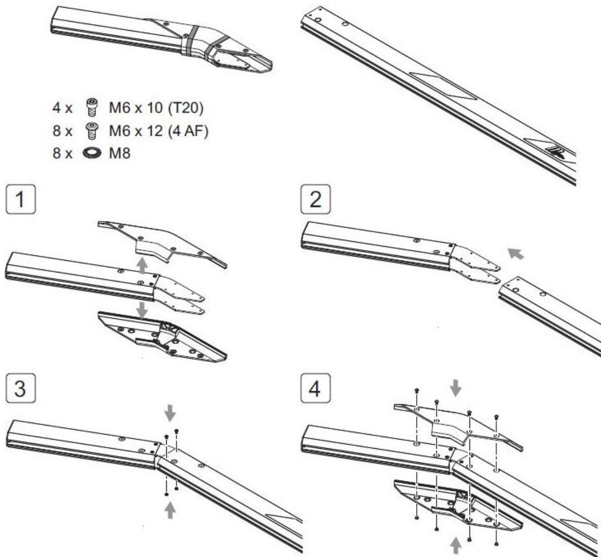
Figure 56. Assembling the Gate Arm
