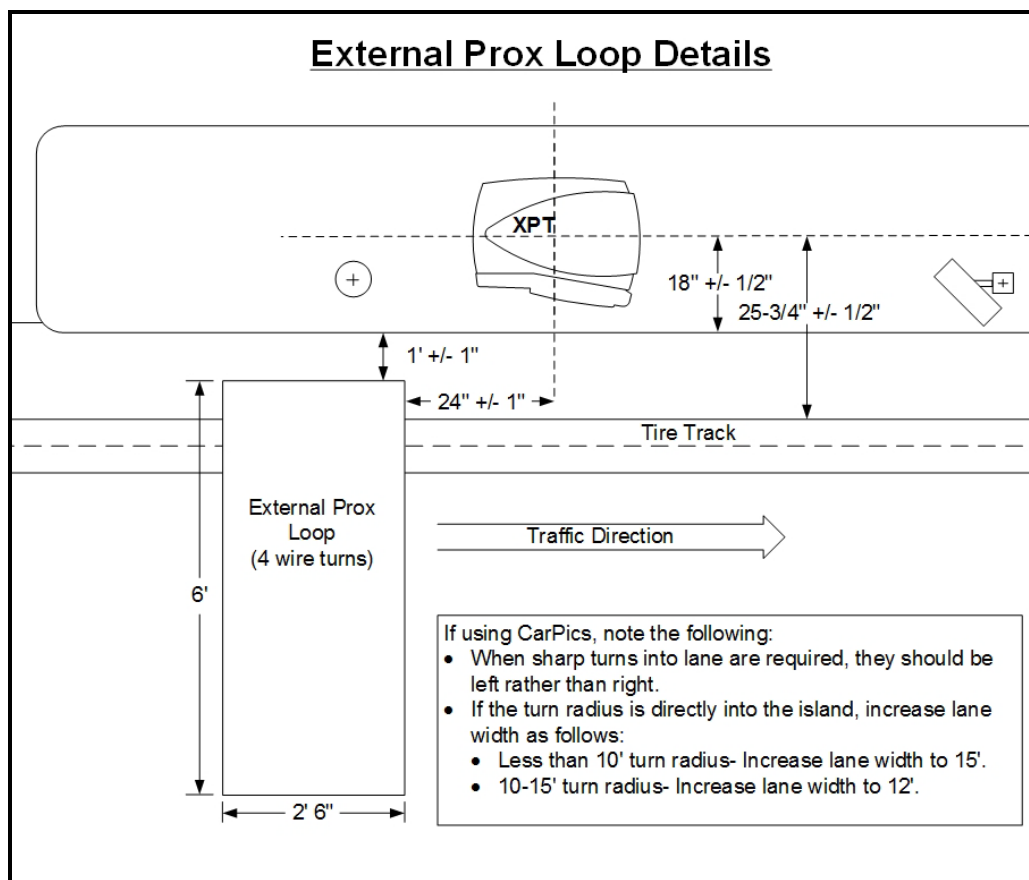
Figure 26. External Prox Loop Details
