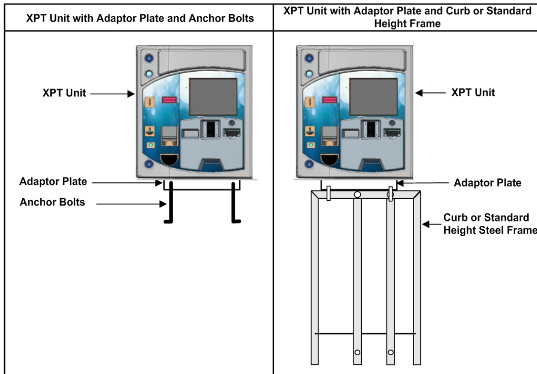
Figure 12. Bricked-In Base Options
