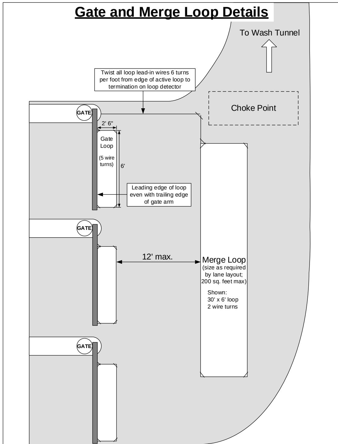
Figure 50. Three XPT Lanes with Single Merge Loop
