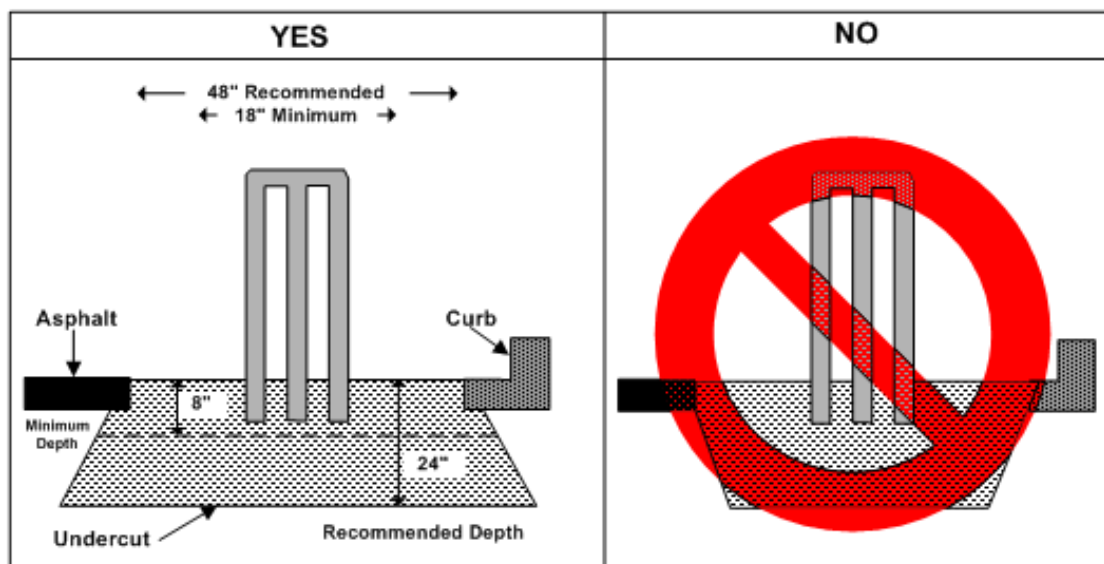
Figure 8. Concrete Pad Dimensions
