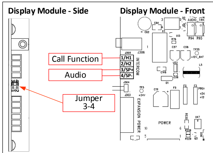
Figure 33. Three-Wire Intercom Configuration
