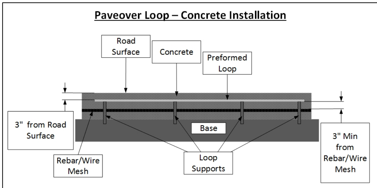
Figure 54. Pave-over Loop - Concrete Installation
