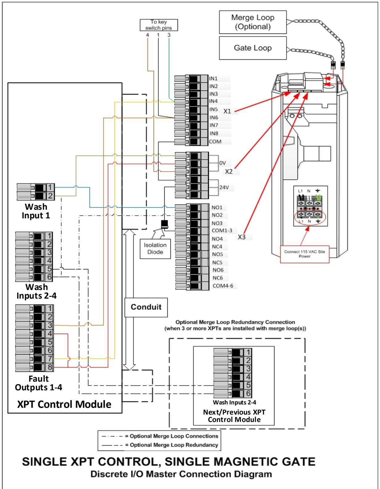
Figure 48. Single XPT Control, Single Magnetic Gate
