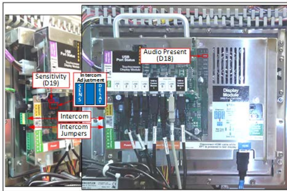
Figure 30. Intercom Component Locations on the Display Module
