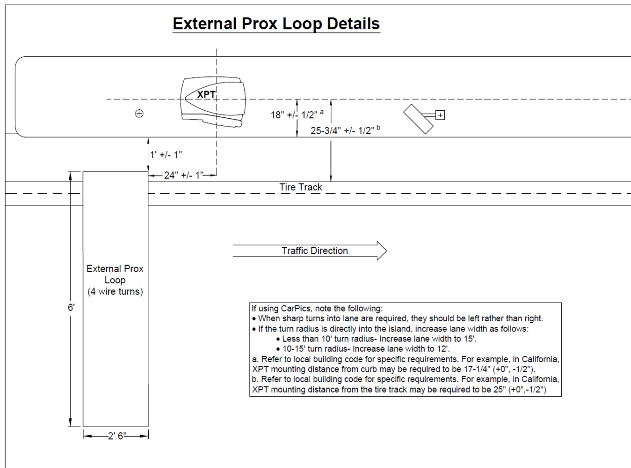
Figure 25. External Prox Loop Details
