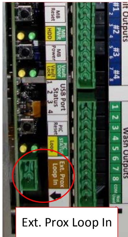
Figure 28. External Prox Loop Lead-In Connections
