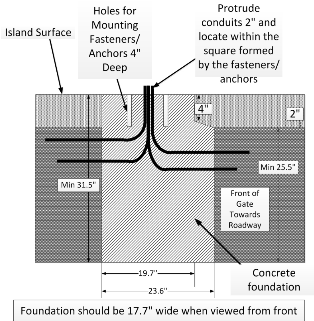
Figure 42. Magnetic Base Side View
